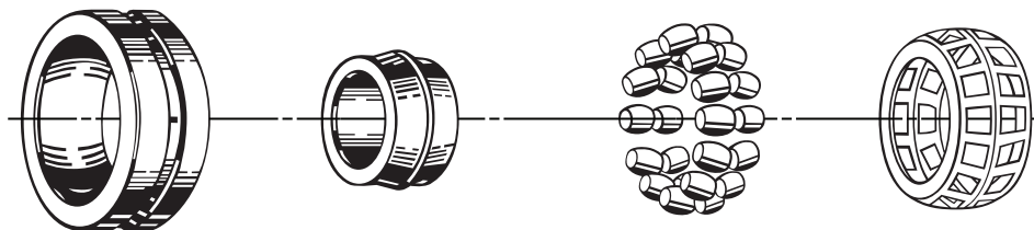
SPHERICAL ROLLERS
